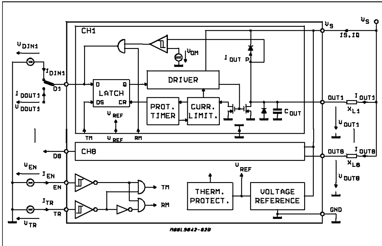
Figure 4 : Test Circuit.
